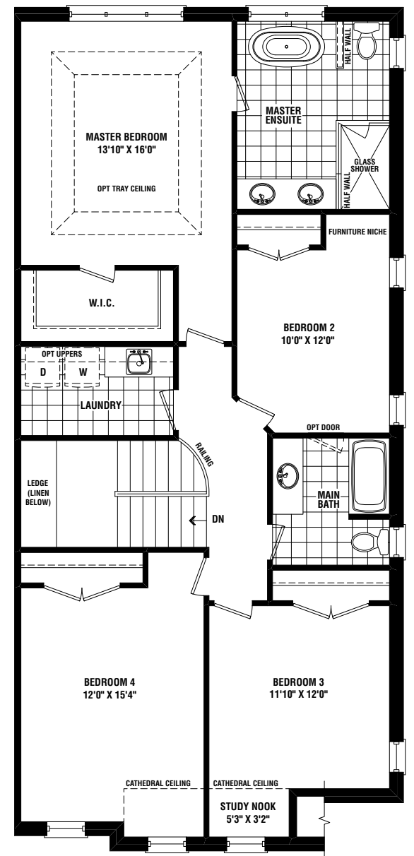
SECOND FLOOR ELEV. 'A-1' OPT. 4 BEDROOM END CONDITION
